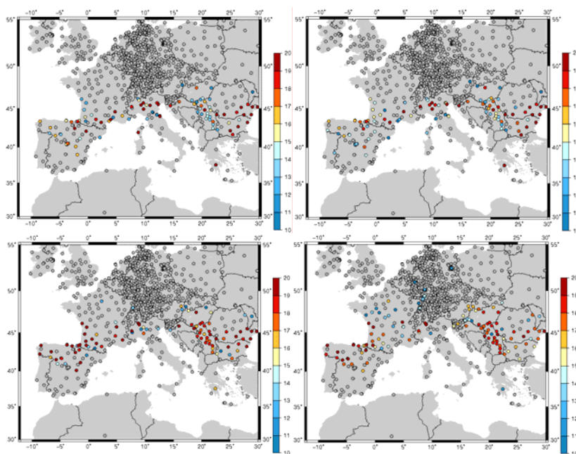
Figure 3: Shown are the number of years, in a 20 year time span, in which the average growing season temperature is within the bounds specified in Table 1 for Merlot noir. Grey circles show stations outside these bounds. The time spans used are 1961-1980 (upper left), 1971-1990 (upper right), 1981-2000 (lower left) and 1991-2010 (lower right).
