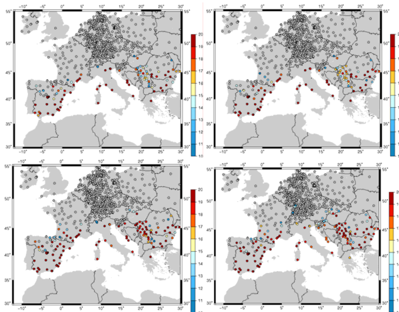
Figure 1: Shown are the number of years, in a 20 year time span, in which the Huglin index exceeds the 1900 threshold (associated with Merlot noir). The time spans used are 1961-1980 (upper left), 1971-1990 (upper right), 1981-2000 (lower left) and 1991-2010 (lower right). Grey circles show stations that fail to exceed the threshold ten times or more.
