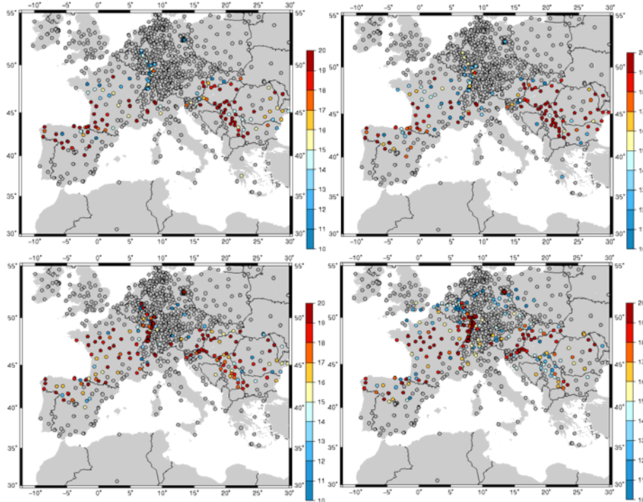
Figure 2: Shown are the number of years, in a 20 year time span, in which the average growing season temperature is within the bounds specified in Table 1 for Sauvignon blanc. Grey circles show stations outside these bounds. The time spans used are 1961-1980 (upper left), 1971-1990 (upper right), 1981-2000 (lower left) and 1991-2010 (lower right).
